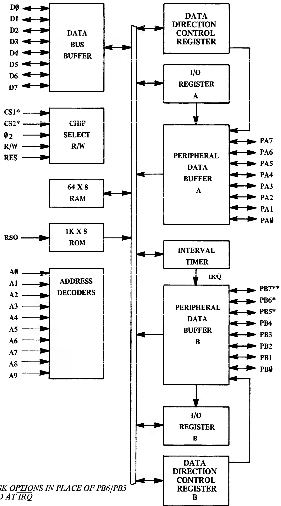
MCS6530 Internal Architecture
